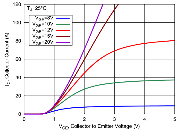
Figure 2. Output Characteristics
