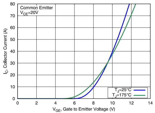
Figure 4. Transfer Characteristics
