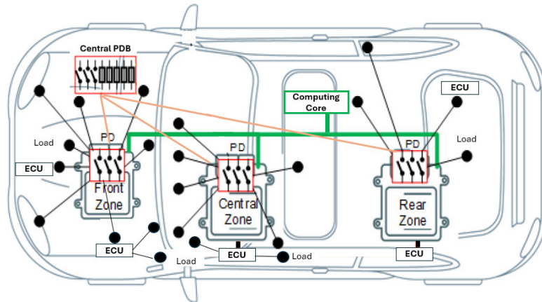
Figure 2. Power Distribution in Zonal Control Architecture
