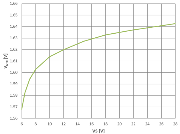
Figure 7. NTC Voltage vs. Supply Voltage ( T_{pcb} = 25^{\circ}\text{C} )
