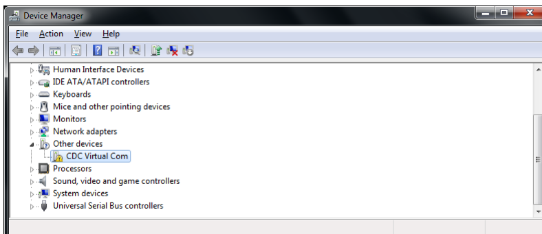
Figure 12. Device Manager
