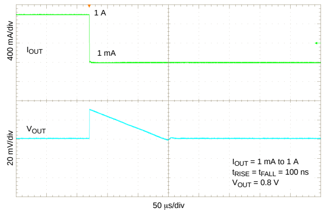
Figure 36. Load Transient Response – 1 A to 1 mA/100 ns
