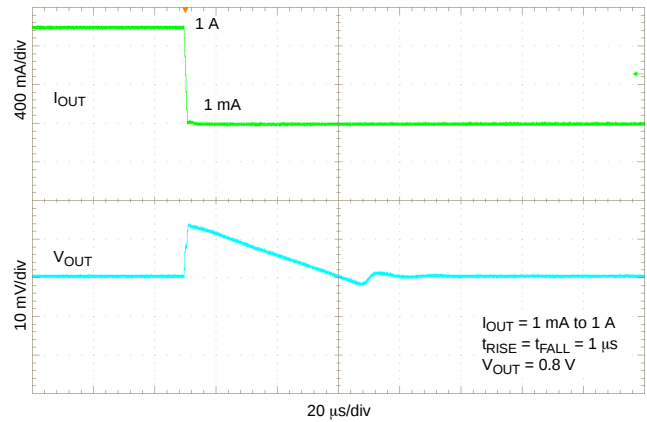
Figure 34. Load Transient Response – 1 A to 1 mA/1 \mu\text{s}
