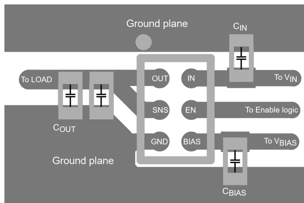
Figure 42. Recommended PCB Layout
