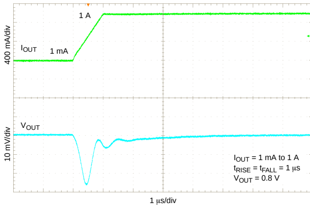
Figure 33. Load Transient Response – 1 mA to 1 A/1 \mu\text{s}
