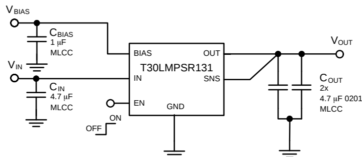
Figure 1. Application Schematic
