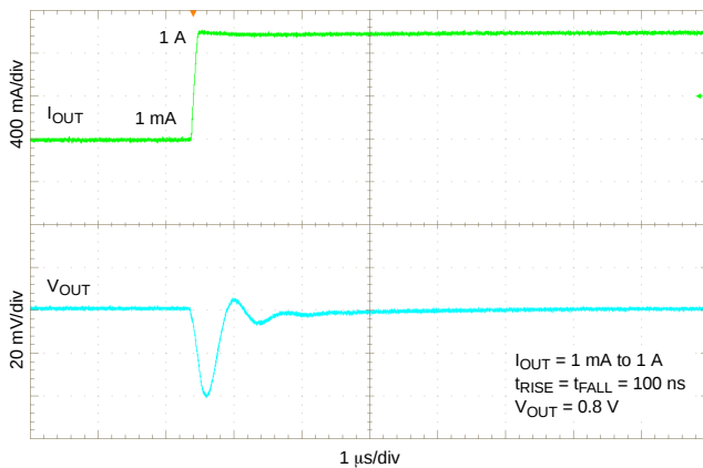
Figure 35. Load Transient Response – 1 mA to 1 A/100 ns
