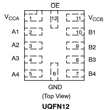
Figure 2. Pin Assignments (Top View)
